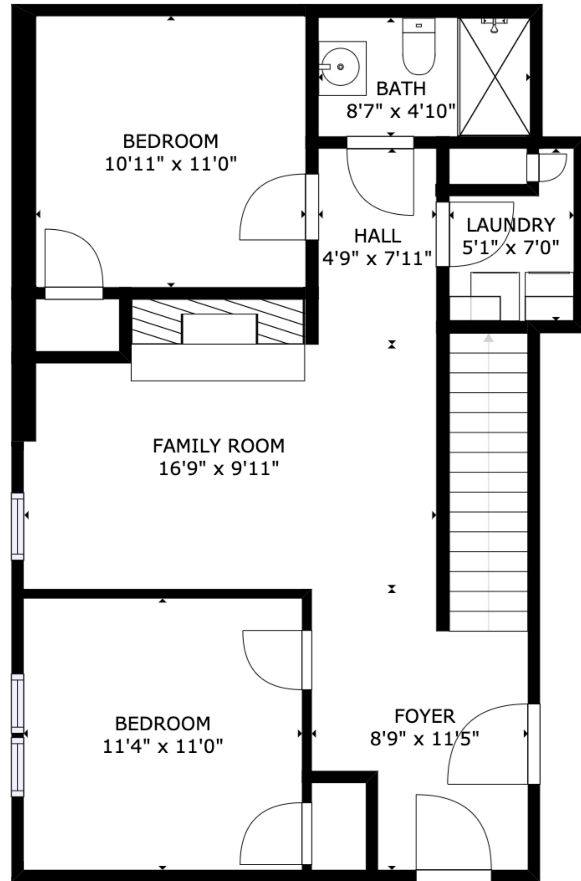
FLOOR 1
