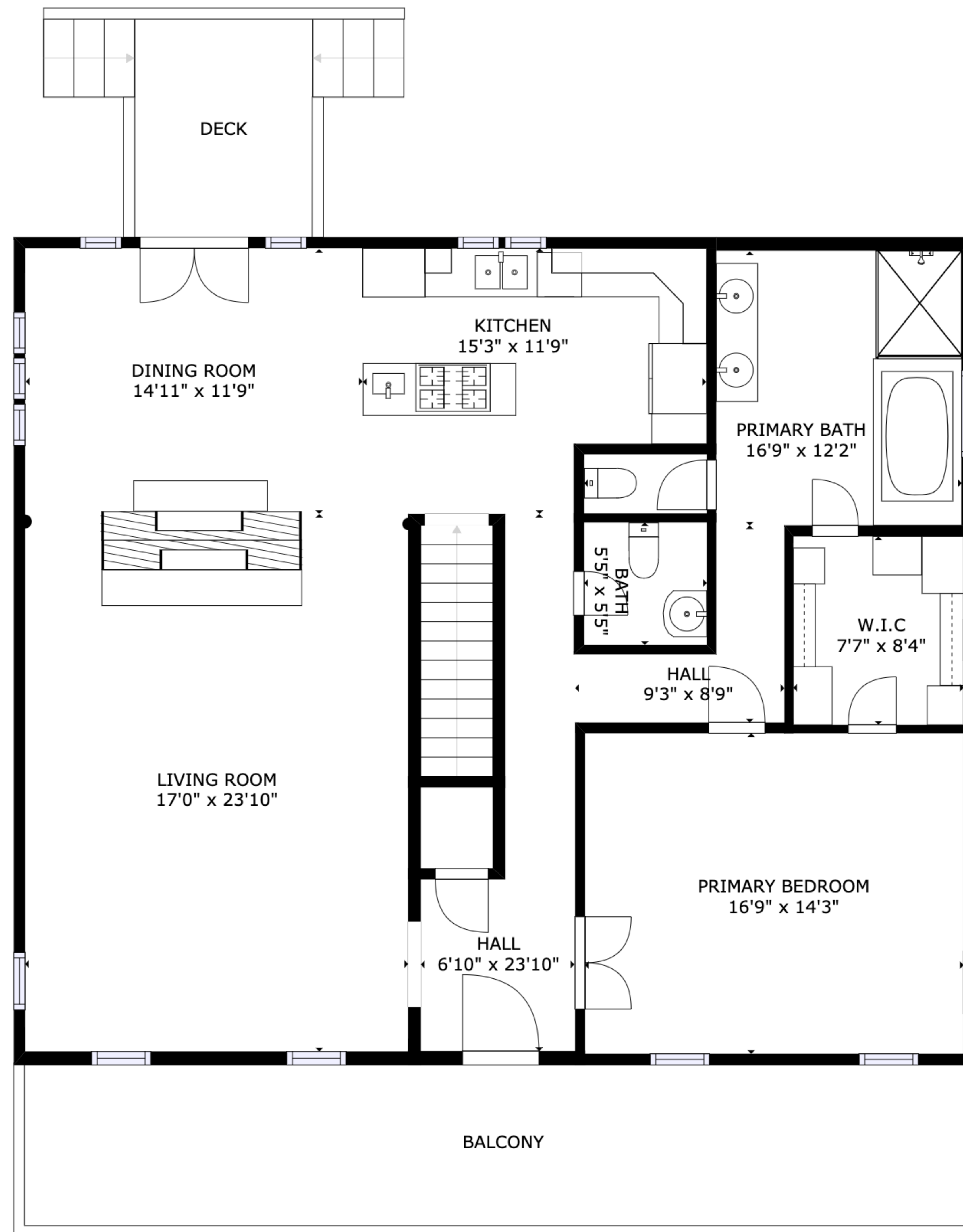
FLOOR 2
